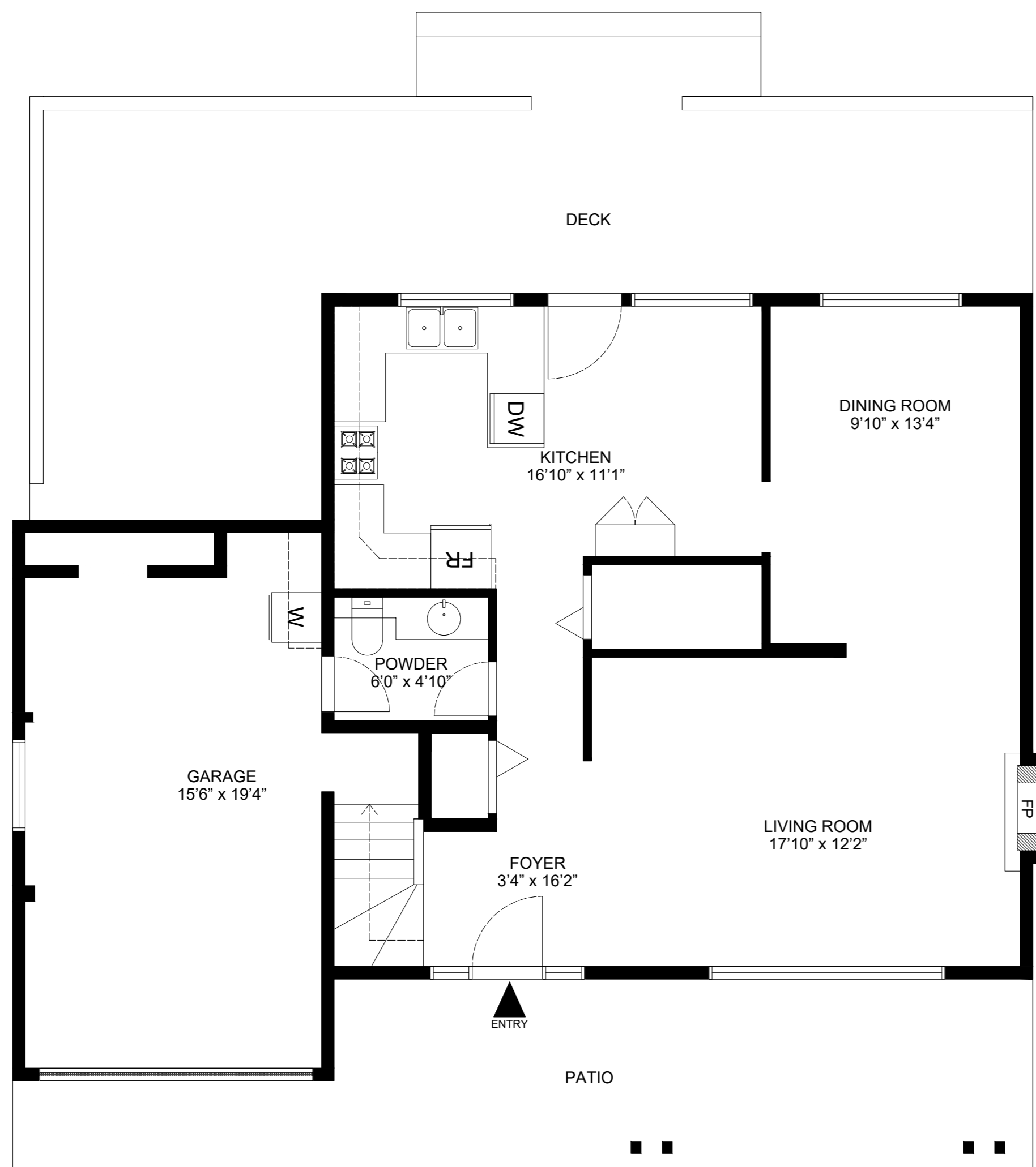
MAIN LEVEL
