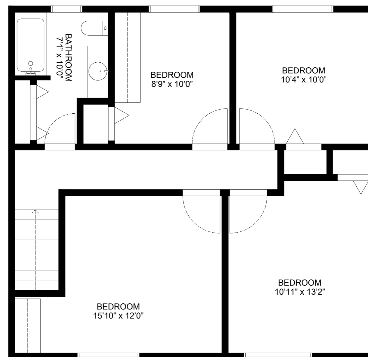
UPPER LEVEL
